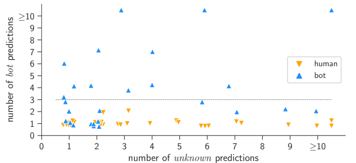
Fig. 2: Accounts predicted as bot/unknown vs ground truth
